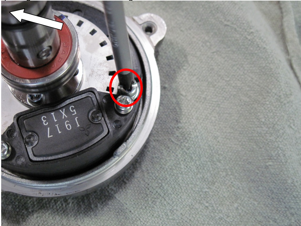
Figure 39: Reinstallation of CAS sensor screws
