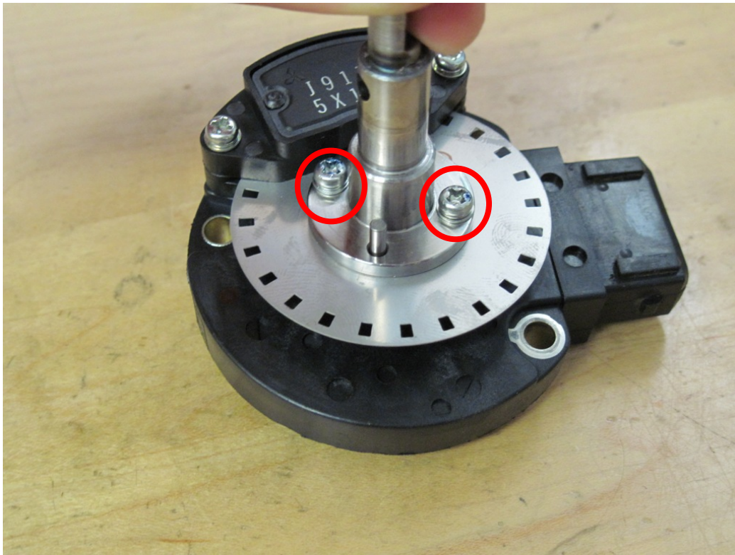
Figure 35: Screws for CAS shaft replaced
