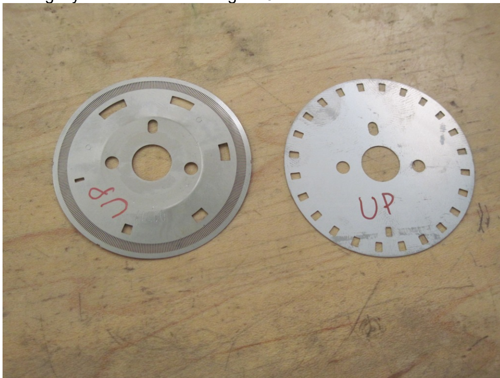
Figure 32: Comparison of original and AEM trigger discs
