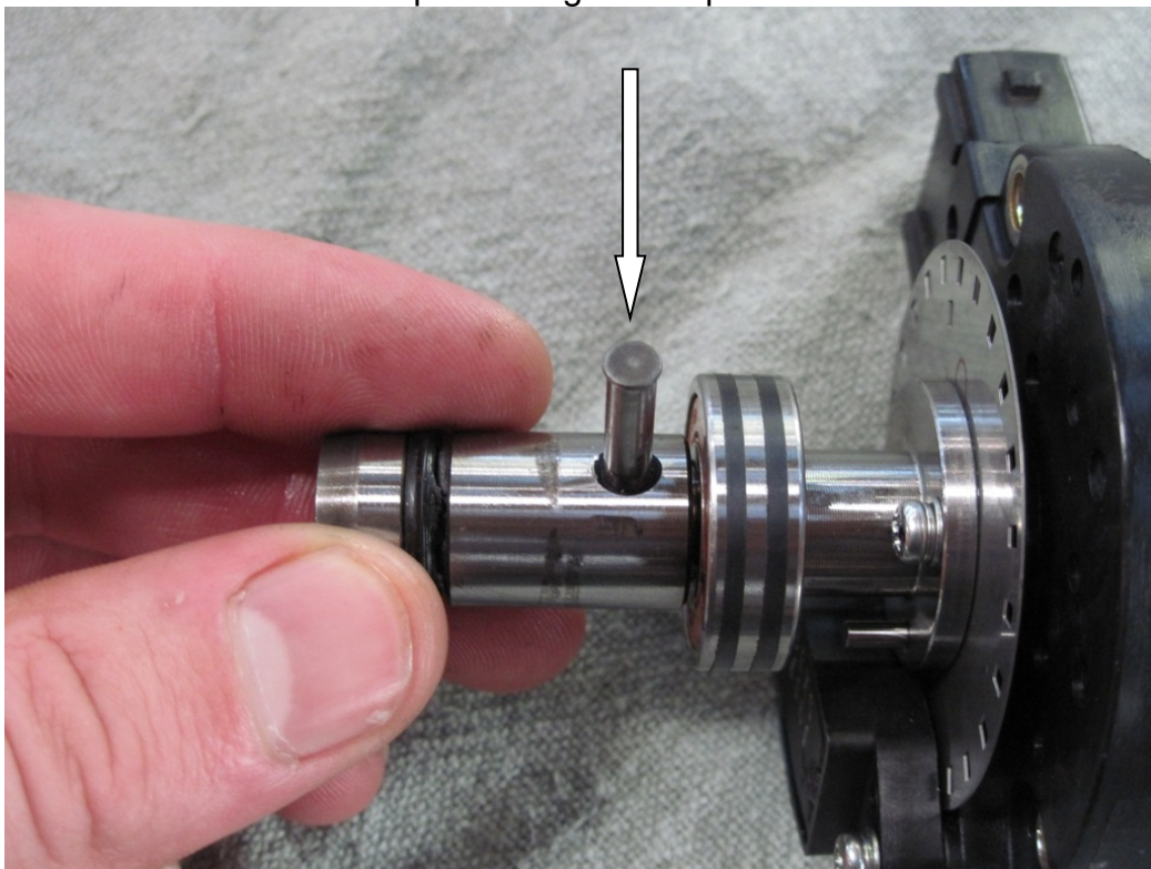
Figure 38: Aligning the star socket retaining pin
