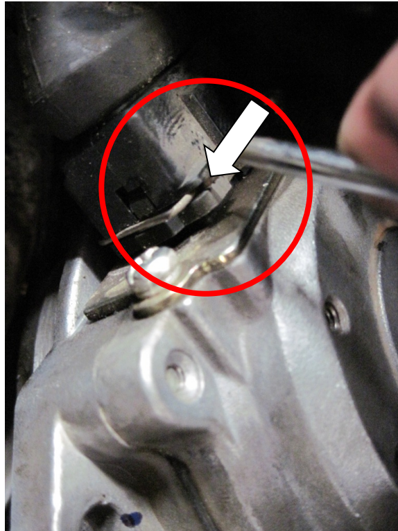
Figure 9: Pry here to remove this clip
