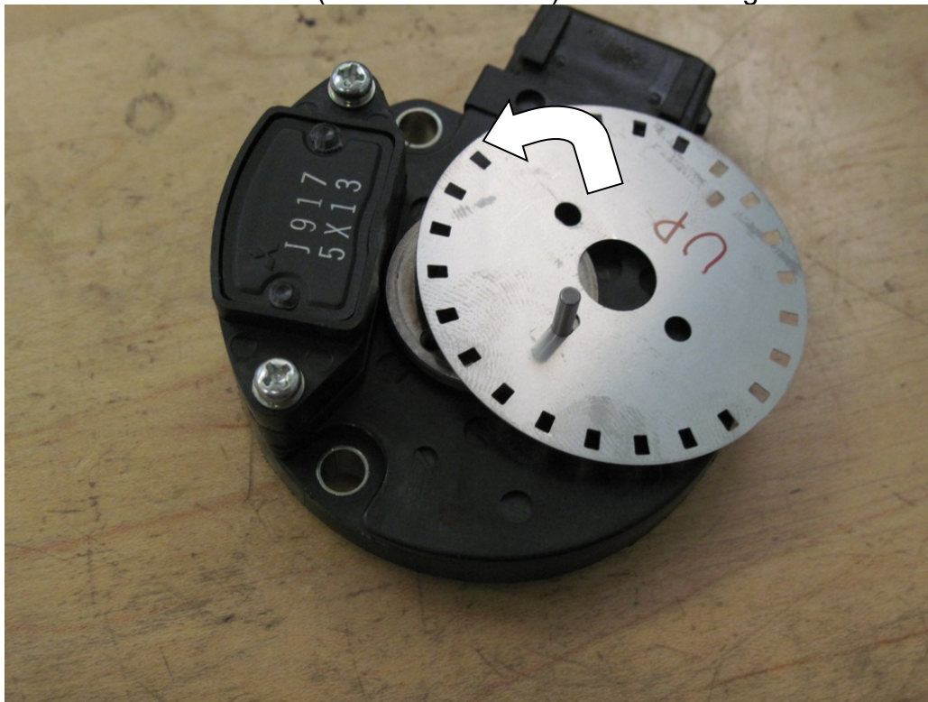
Figure 33: AEM trigger disc being installed
