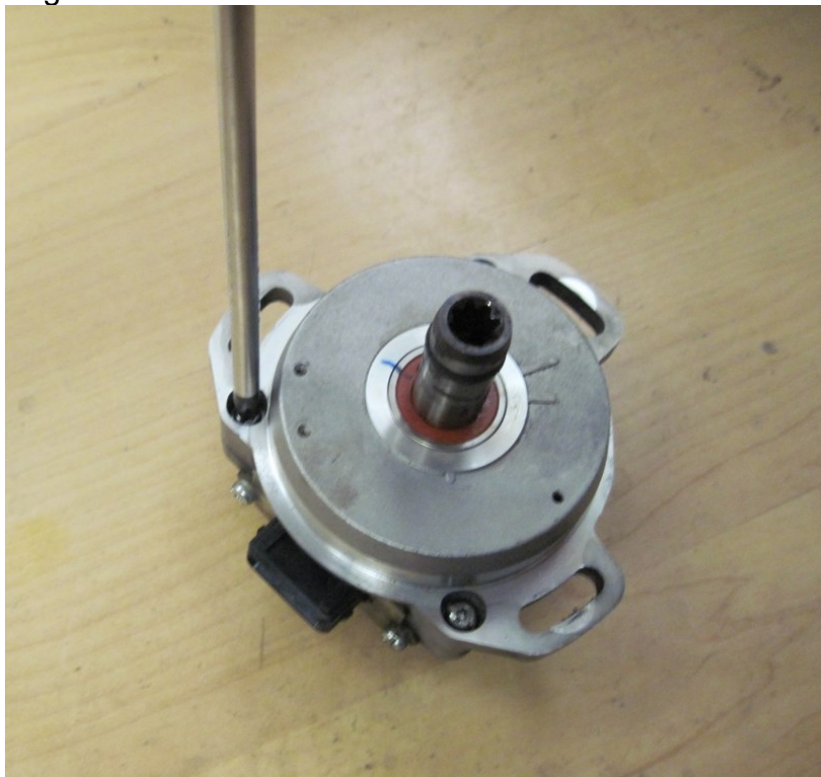
Figure 14: Taking apart CAS assembly using number 2 Phillips screwdriver
