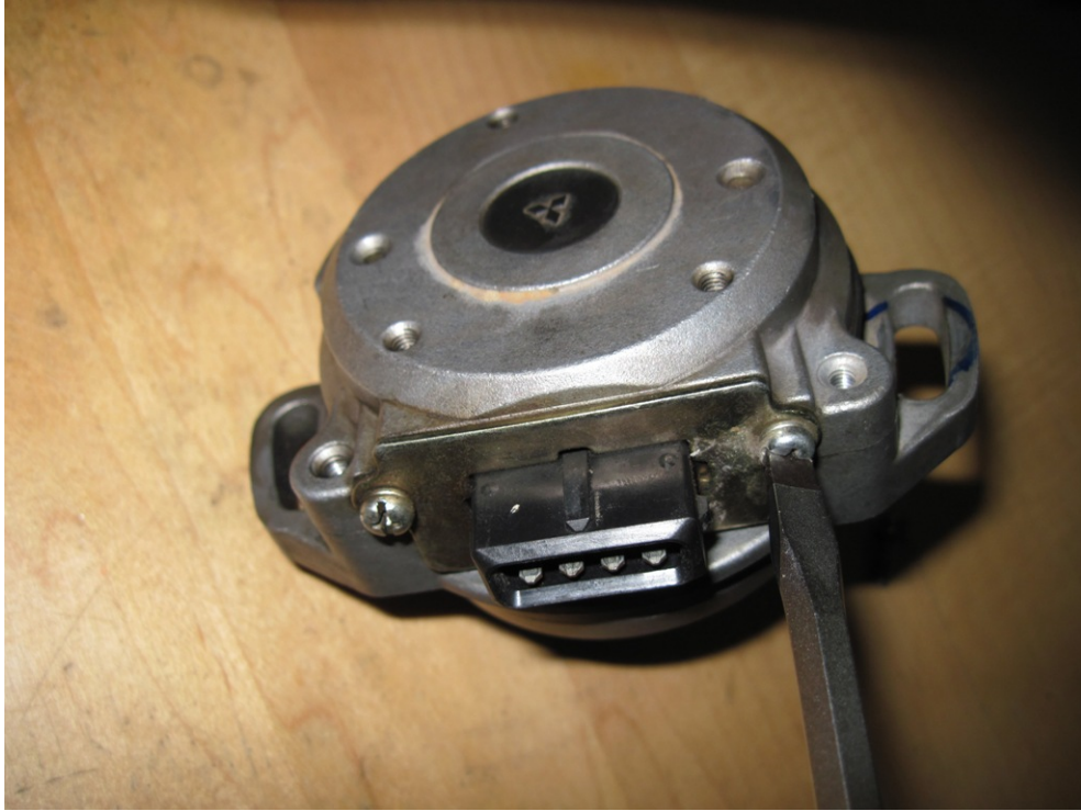
Figure 15: Removing seal cover on CAS assembly using ¼" screwdriver
