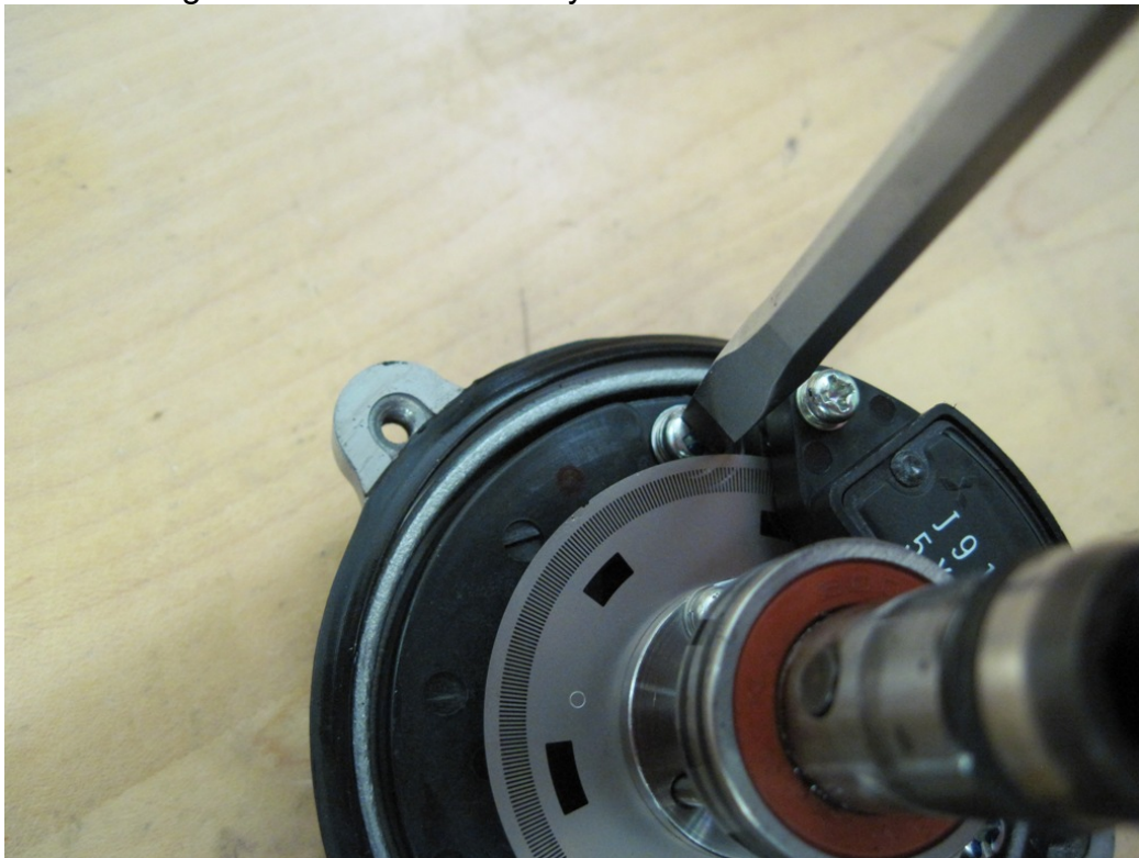
Figure 18: Remove 3 screws holding sensor using 1/4" flat screwdriver
