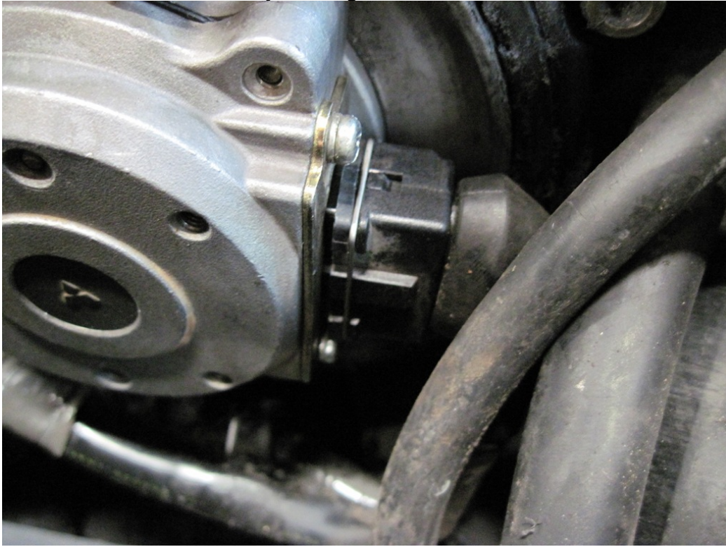
Figure 45: Replacing CAS sensor connector
