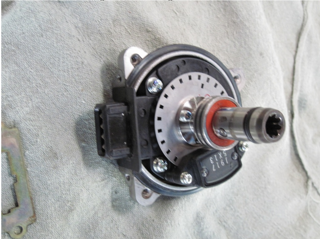
Figure 40: CAS rubber seal reinstalled
